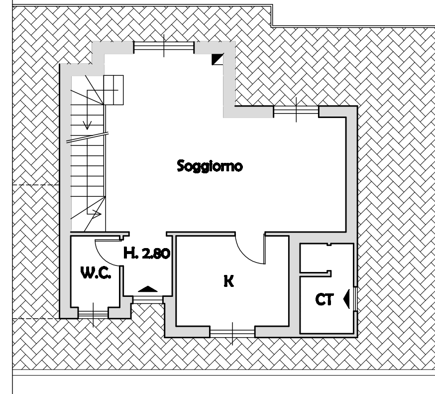
Piano Terreno
