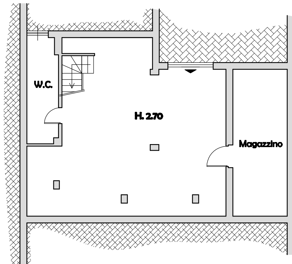
Piano Seminterrato
